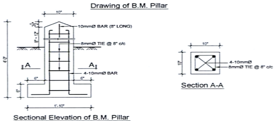
Map 5-1: BM pillar design
